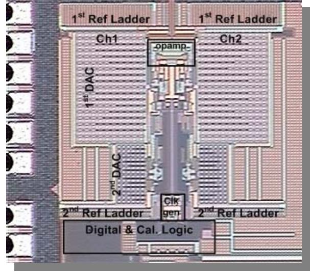
Fig. 5: Chip micrograph.
