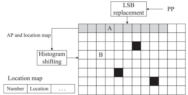
Fig. 3. Image segmentation and self-embedding in pixel shrink, where black pixels represent that their pixel values satisfy I_{i,j} \geq 250 .
