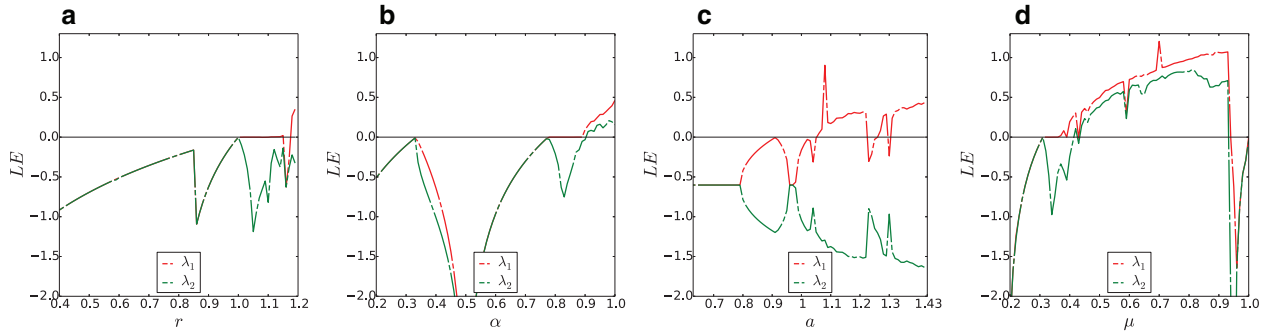
Fig. 3. LEs of different 2D chaotic maps: (a) 2D Logistic map; (b) 2D-SLMM with parameter \beta = 3 ; (c) Hénon map with parameter b = 0.3 ; 2D-LASM.
