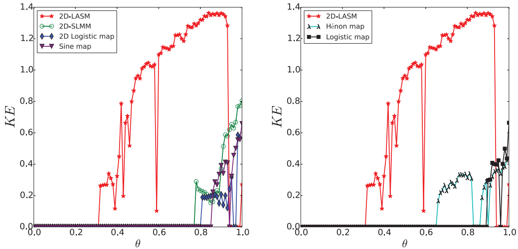
Fig. 4. KEs of different chaotic maps, where parameter \theta denotes \mu, \alpha, r - 0.2, a - 0.4, p and s for 2D-LASM, 2D-SLMM, 2D Logistic map, Hénon map, Logistic map and Sine map, respectively.
