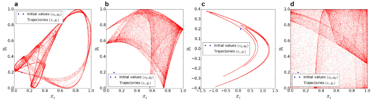
Fig. 2. Trajectories of different 2D chaotic maps: (a) 2D Logistic map with parameter r = 1.19 ; (b) 2D-SLMM with parameters \alpha = 1, \beta = 3 ; (c) Hénon map with parameter a = 1.4, b = 0.3 ; (d) 2D-LASM with parameter \mu = 0.9 .
