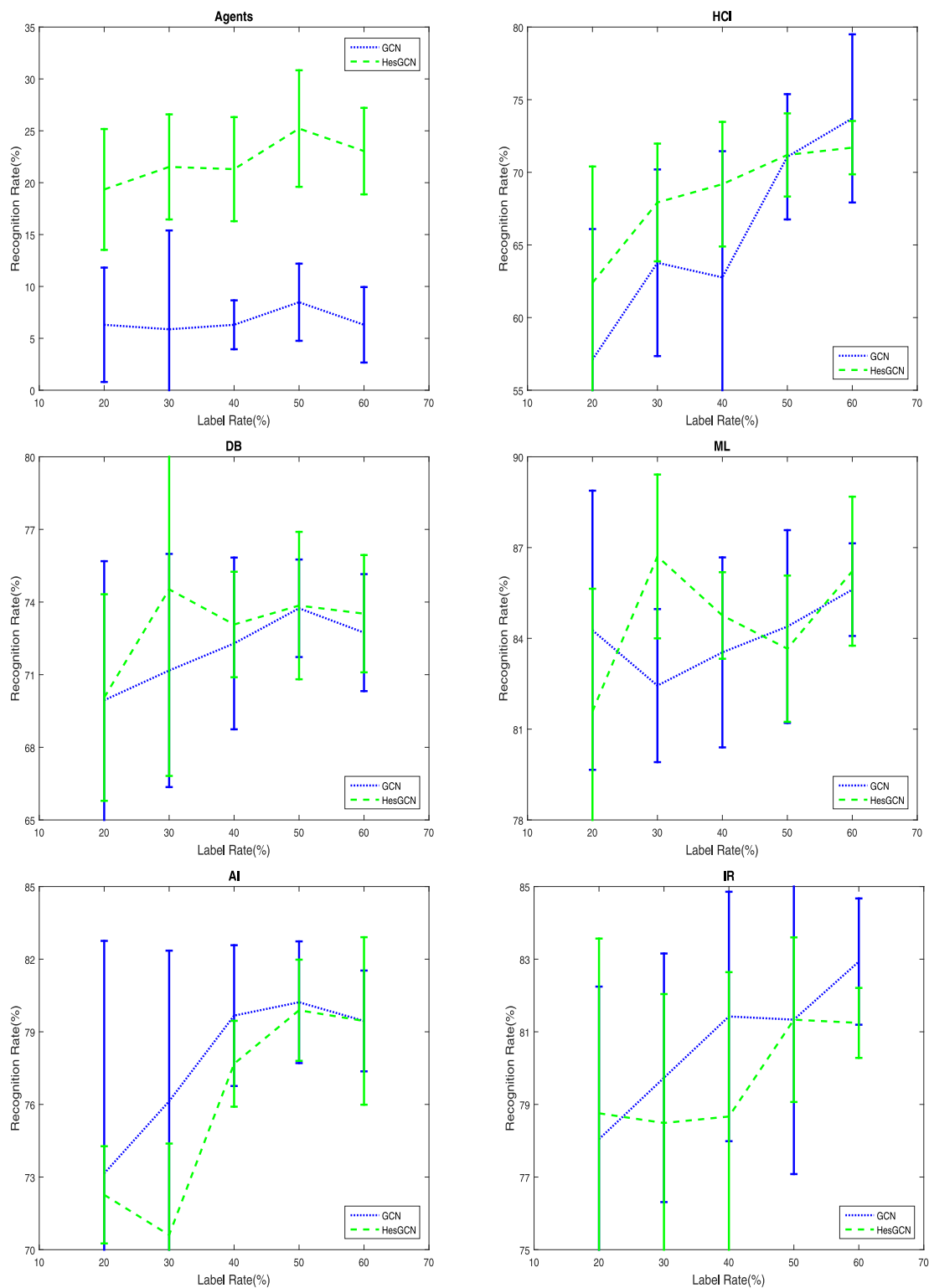
Fig. 4. Recognition accuracy of each class in the Citeseer database, including Agents, AI, DB, IR, ML, HCI. Each subfigure corresponds on single class.
