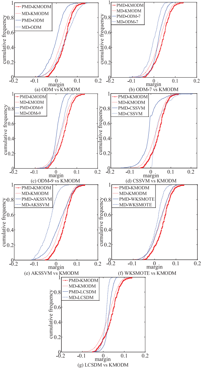
Fig. 5. Cumulative frequency (y-axis) with respect to margin (x-axis) of ODM, ODM-7, ODM-9, CSSVM, AKSSVM, WKSMTM, LCSDM and KMODM on German data set using RBF kernel.
