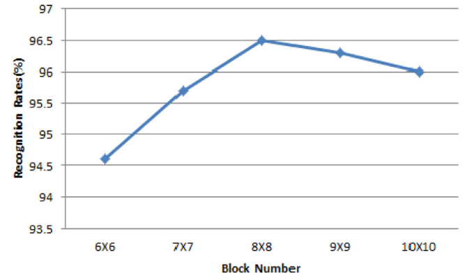
Fig. 8. The recognition rates versus block number upon the FERET database.
