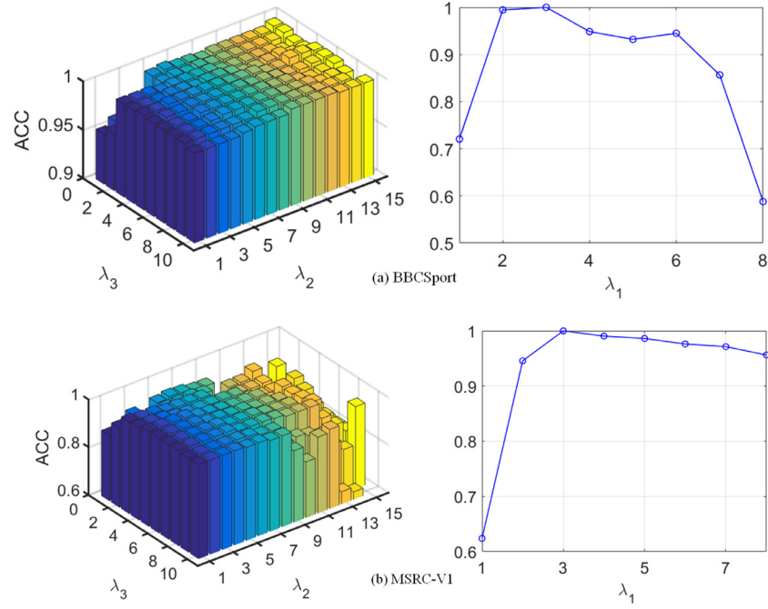
Fig. 4. ACC values of GLTA with different combinations of \lambda_2 and \lambda_3 by fixing \lambda_1 on (a) BBCSport and (b) MSRC-V1 datasets.
