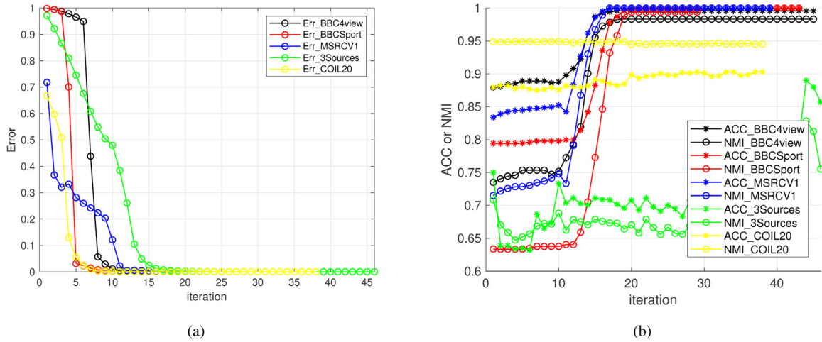
Fig. 5. (a) Empirical convergence versus iterations; (b) ACC and NMI versus iterations.
