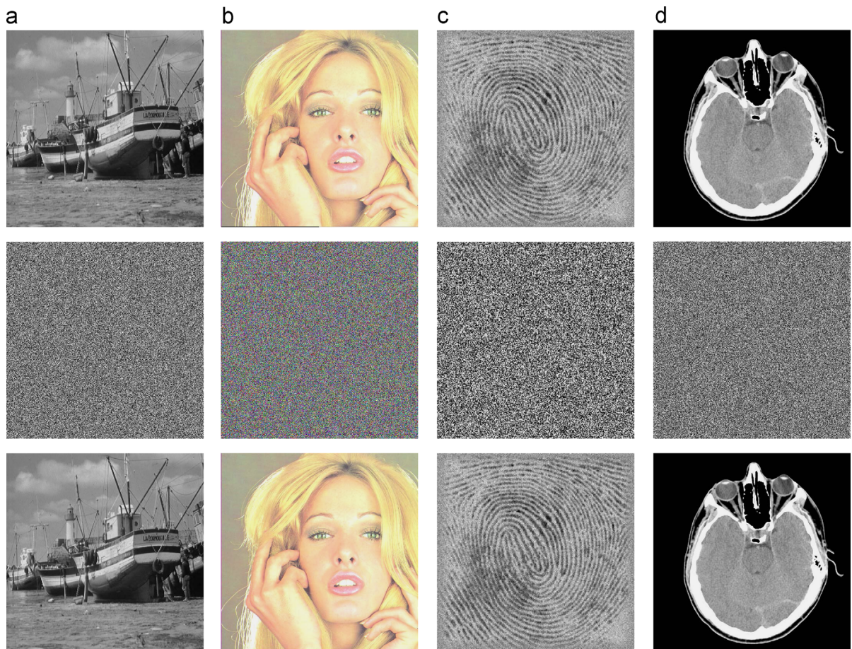
Fig. 5. Encrypting different images using the proposed PSCS-IE algorithm. The top, middle and bottom rows show the original, encrypted, reconstructed images, respectively. (a) grayscale image; (b) color image; (c) fingerprint (biometrics); (d) medical image.
