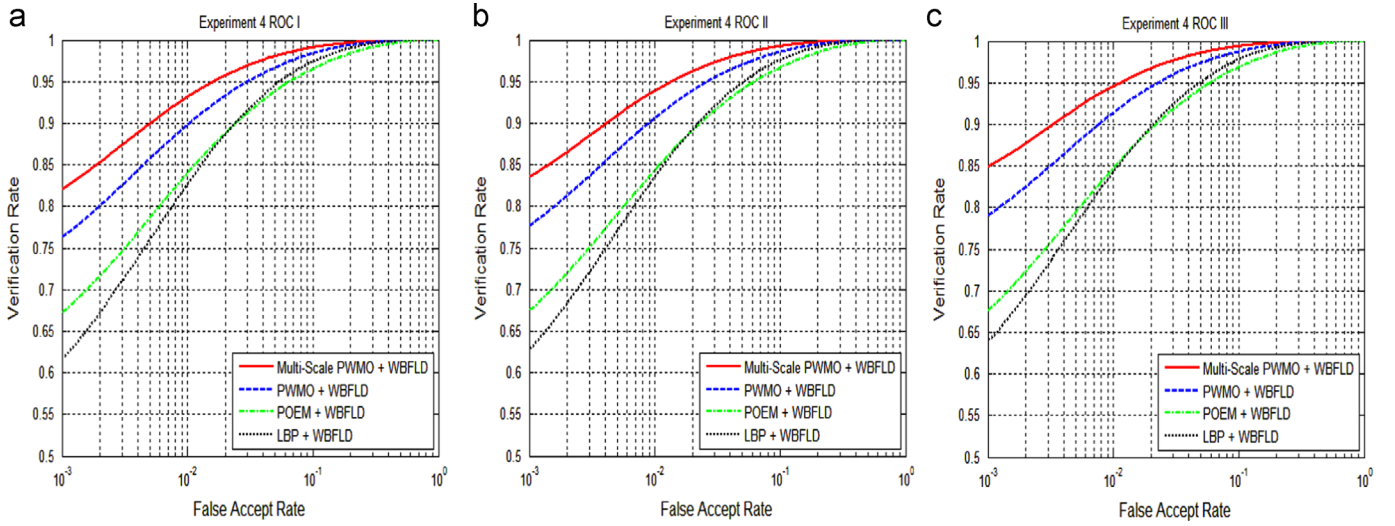
Fig. 16. ROC curves corresponding to the LBP, POEM, PWMO and multi-scale PWMO based face representation approaches on FRGC2.0 Experiment 4: (a) ROC I. (b) ROC II. (c) ROC III.
