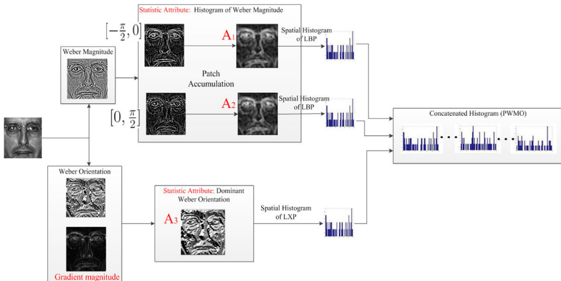
Fig. 7. An illustration of the framework based on PWM for face representation.
