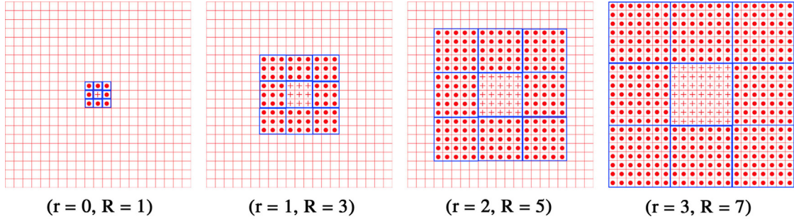
Fig. 8. Illustration of multi-scale PWMO for different (r, R) .
