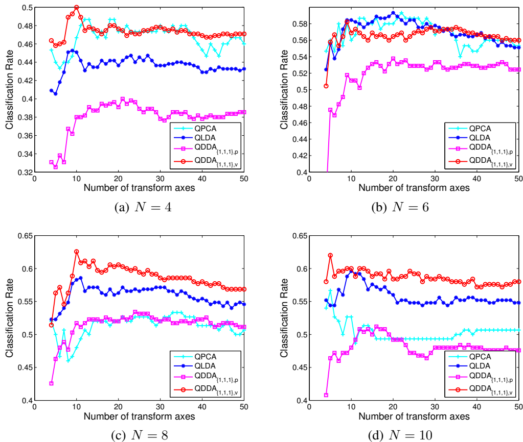
Fig. 4. Classification accuracies of QDDA, QPCA, and QLDA on the normalized GTFB color face database with different numbers of the training samples.
