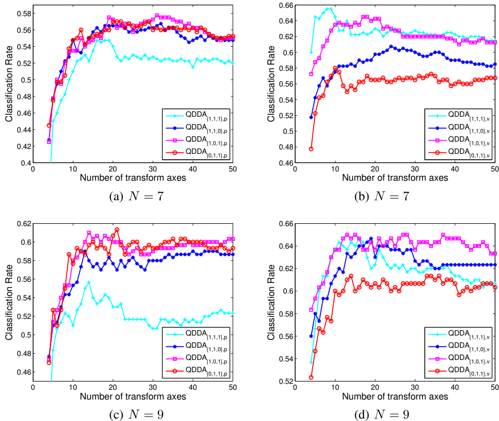
Fig. 3. Classification accuracies of QDDA using parallel and vertical components of QR of color images. (a) and (b) are the results of QDDA_{\{\bullet\},p} and QDDA_{\{\bullet\},v} with N = 7 , and (c) and (d) are corresponding results of N = 9 .
