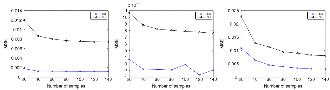
Fig. 5.1. Empirical comparison of g(x) = \sin(\pi x) and \sigma_\epsilon = 0.01, 0.05, 0.25 .
