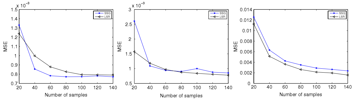
Fig. 5.2. Empirical comparison of g(x) = x^2 and \sigma_\epsilon = 0.01, 0.05, 0.25 .
