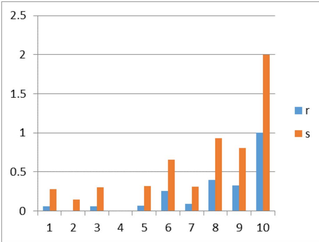
Fig. 4. Sum of sparse parameter r_1^c and the superimposed SSP score vector s_1^c in the second iteration.
