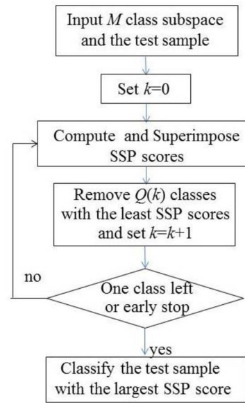
Fig. 2. Flow chart of the FSSP classifier.
